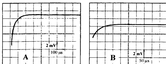
Fig. 6. Time-evolution of the laser-induced open-circuit photopotential. (A) Solution 10^{-2}\text{ M} in \text{Ru}(\text{TAP})_3^{2+} , 10^{-2}\text{ M} in \text{H}_2\text{Q} , 2 \times 10^{-5}\text{ M} in BQ and 5 \times 10^{-2}\text{ M} in \text{LiNO}_3 . (B) Same as (A) but with 4 \times 10^{-5}\text{ M} BQ. Dark \text{SnO}_2 potential = +0.28\text{ V/SCF} [adapted from Ref. [43]].
