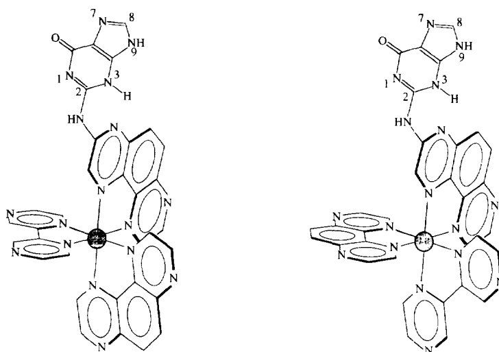
Fig. 12. Structures of the photoadducts formed under irradiation of \text{Ru}(\text{bpy})_3^{2+} in the presence of DNA, after enzymatic and acid hydrolytic treatments of the photosensitized DNA.
