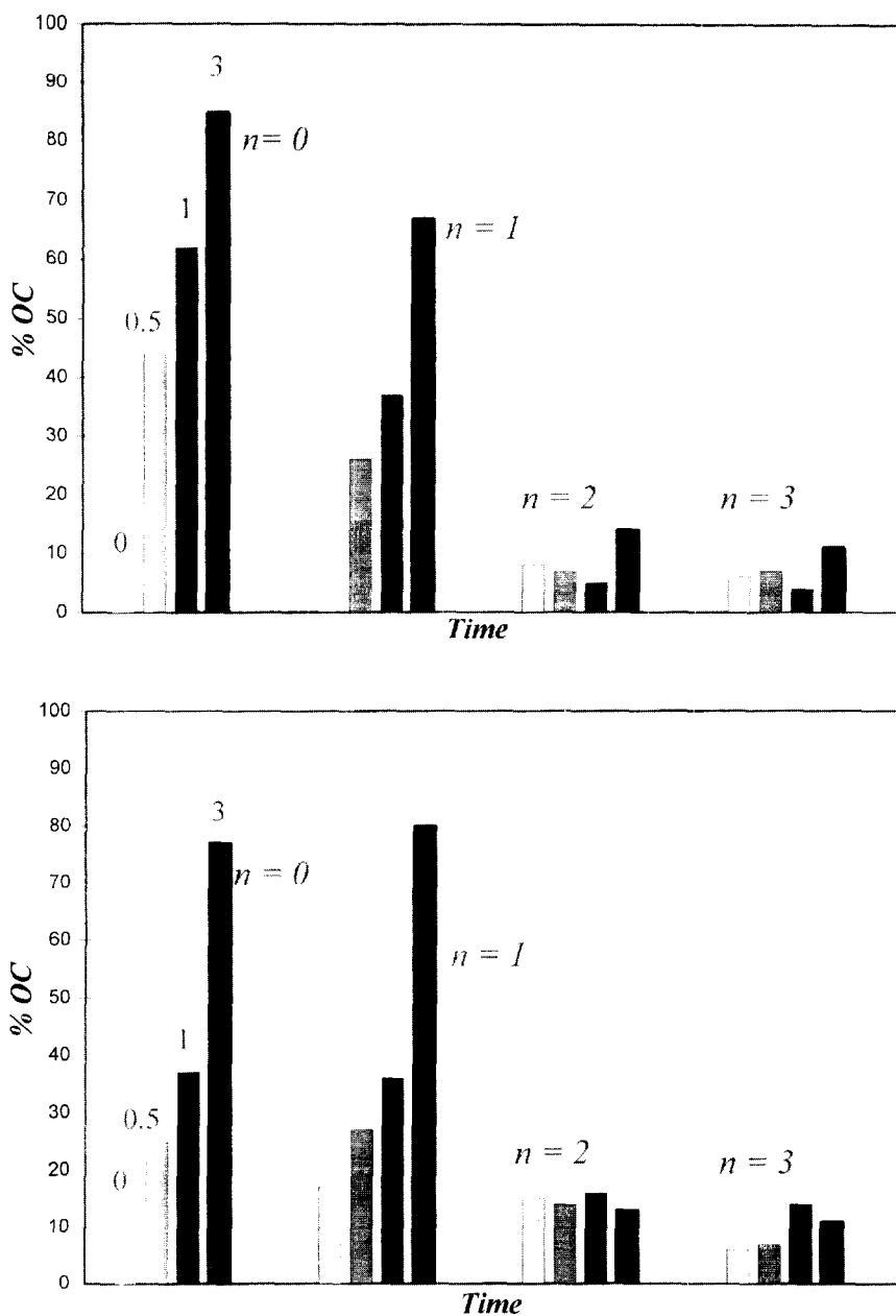
Fig. 10. Percentage of OC form on visible irradiation of the plasmid pBR322 in the presence of \text{Ru}(\text{bpy})_3(\text{TAP})_3^{2+} , n = 0, 1, 2, 3 , ( \text{P/D} = 10 in 10 mM phosphate buffer, pH 7), with 0 min (dotted bars), 0.5 min (light hatch bars), 1 min (dark hatch bars) and 3 min (filled bars), of irradiation at 436 nm [adapted from Ref. [46]].
